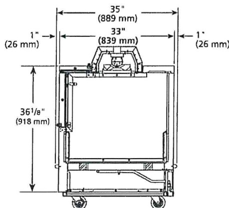
RIGHT VIEW
