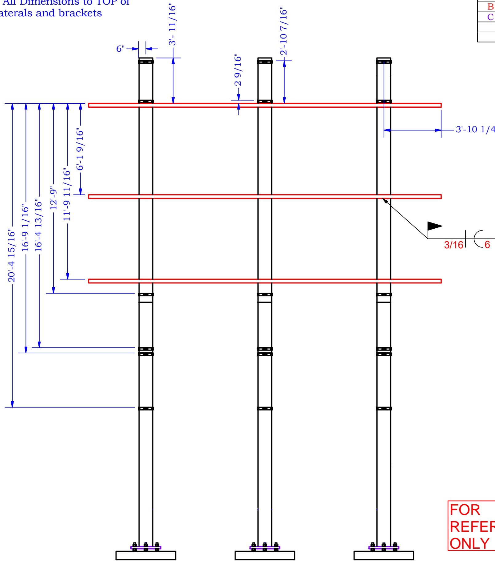
Front View
