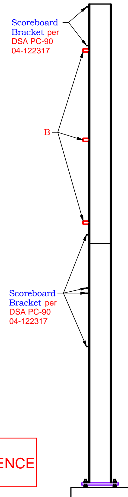
Side View
